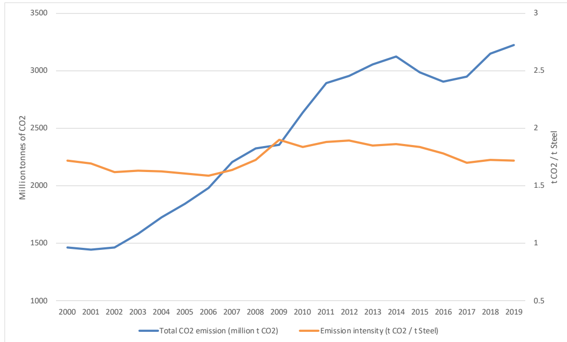
Figure 5. Emissions arising from steelmaking activities, 2000-2019
