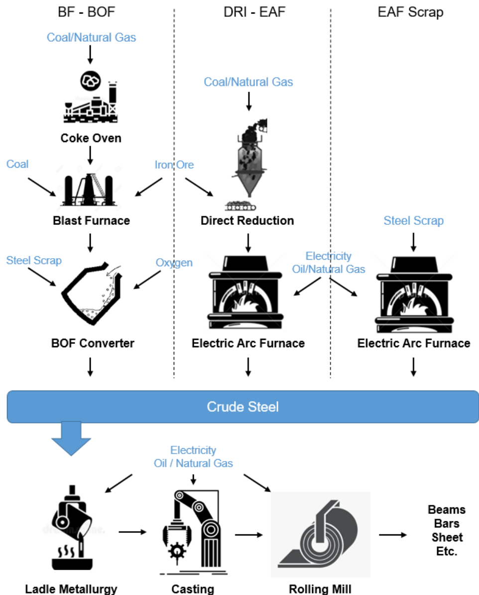
Figure 4. Emissions arising from the steel supply chain
