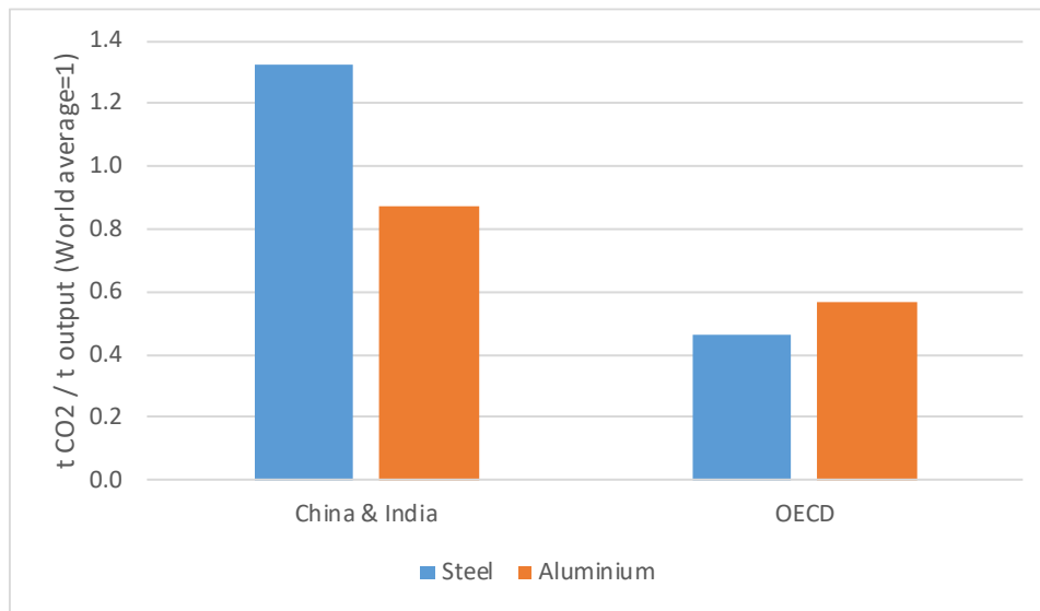
Figure 19. Relative CO 2 intensity of output in steel and aluminium
